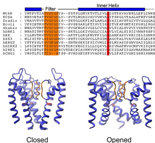
Fig. 2. Closed and opened conformations of the pore. Sequences of ligand- and voltage-gated K^+ channels are from [13]. The selectivity filter sequence is highlighted orange and the glycine gating hinge red. Three subunits of the closed pore conformation of KcsA (left) and the opened pore conformation of MthK (right) are shown with the selectivity filter and gating hinge colored to match the sequence highlights.
